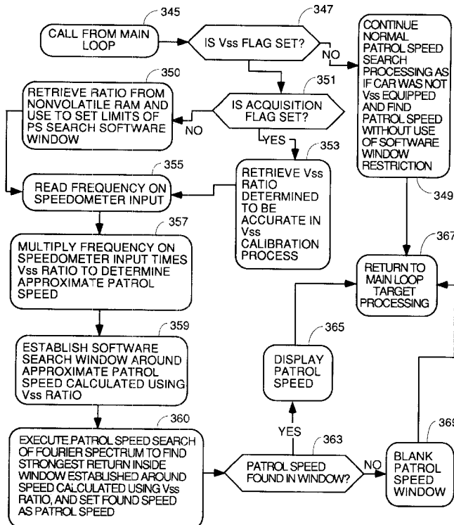
PROCESS TO USE V SS RATIO AFTER CALIBRATION PROCESS COMPLETED - PREFERRED EMBODIMENT
