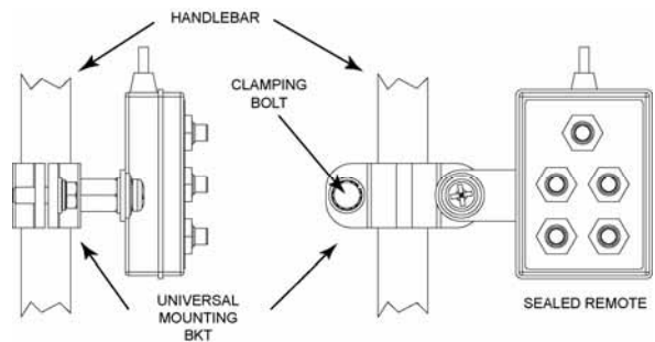
200-0279-00 ñ Sealed Remote 200-0524-00 Universal Mounting Bracket For mounting on handlebars from 3/4" to 1 1/2" in diameter.
